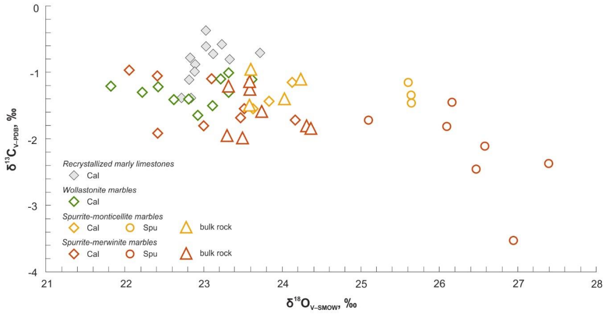
Supplementary Figure 4. C and O isotope compositions of calcite, (CO 3 )-group of spurrite, and bulk samples of marbles and marly limestones (the Kochumdek contact aureole). Cal, calcite; Spu, spurrite.
